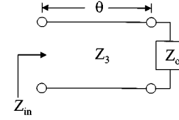
Fig. 4. Simplified model for the microstrip line with the DGS. Z_0 (50 \Omega ) is the system characteristic impedance for the calculation of Z_3 and measurement. Here, Z_0 is attached as a load to calculate Z_3 .
